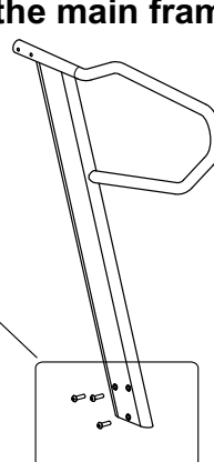
Hex Socket Button Head Screws M10 x 50L x 3 pcs
